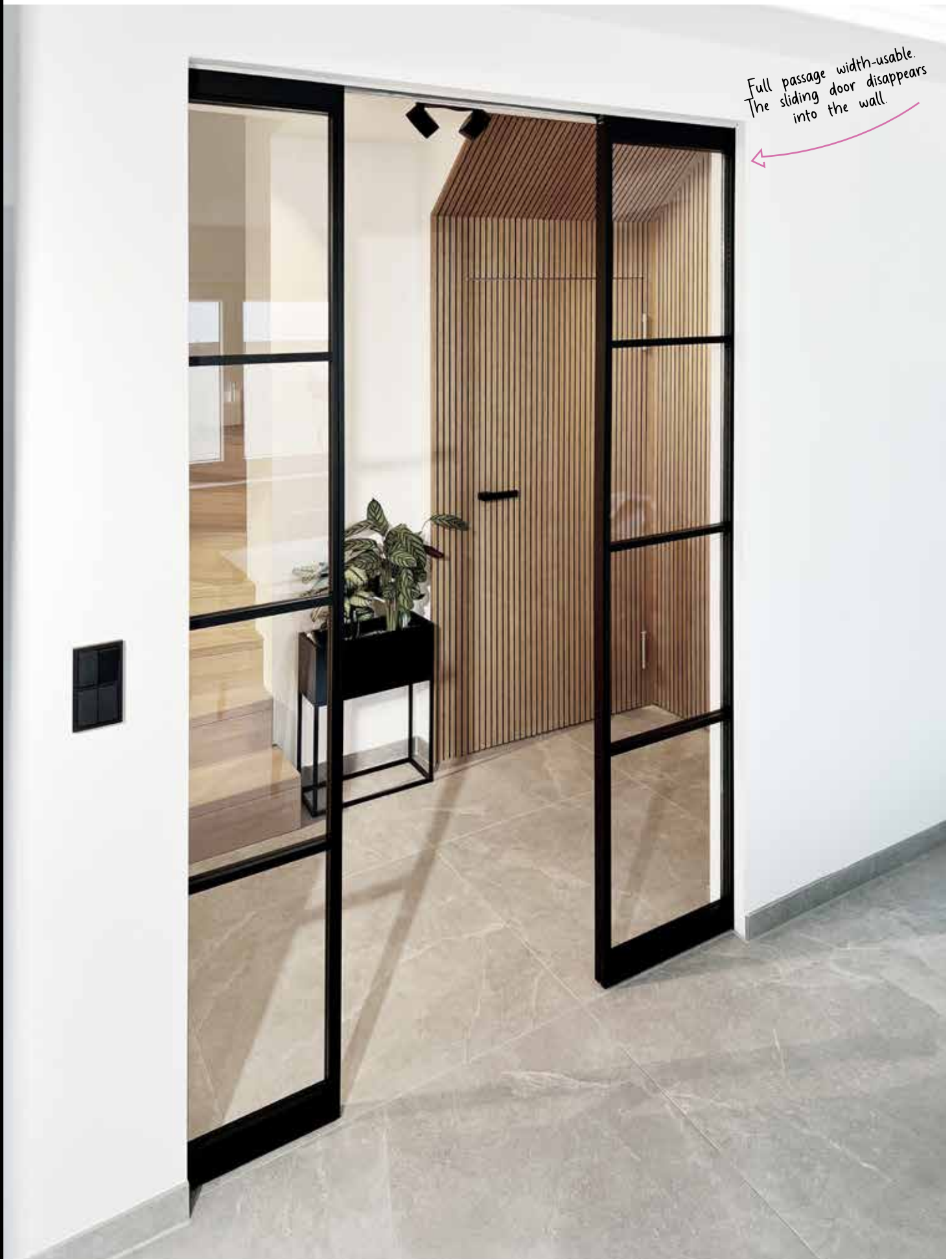
Sliding door running in the wall, 2-panels, Timeless | 3 bars, clear glass | black, RAL 9005, matt, fine texture| without handle
